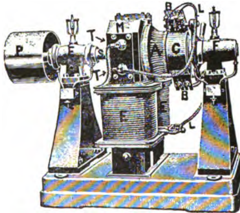
FIG. 428.—A Typical Dynamo-Electrical Generator, with parts lettered. A, the armature; B, B, the brushes; C, the commutator; E, E, the windings of the field magnets; M, the pole piece of the salient field magnet; F, F, bearings of the armature spindle; L, L, the lead wires; P, the pulley; T, T, terminal connections of the outside circuit.
